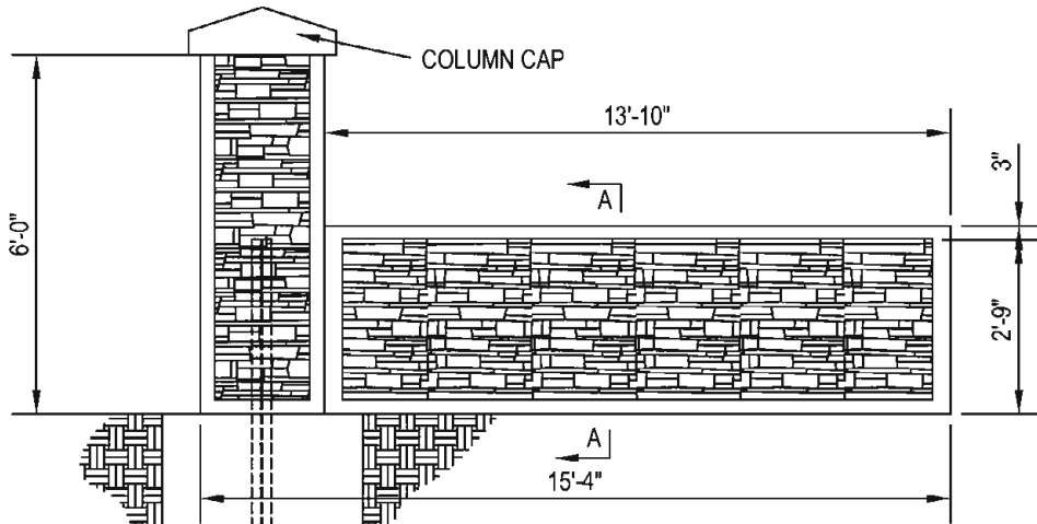
3' PANEL WITH 6' COLUMN FRONT ELEVATION
