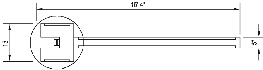
3' PANEL WITH 6' COLUMN TOP ELEVATION
