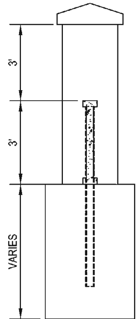
A-A 3' PANEL WITH 6' COLUMN SIDE ELEVATION
