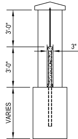
A-A 8' PANEL WITH 8' COLUMN WITH FOUNDATION SIDE ELEVATION
