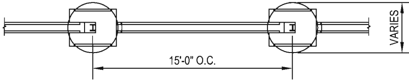
B - 4' PANEL WITH 8' COLUMN WITH FOUNDATION TOP ELEVATION
