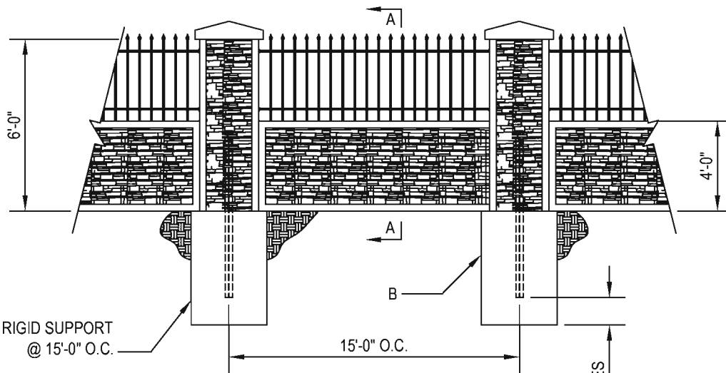
4' PANEL WITH 8' COLUMN WITH FOUNDATION FRONT ELEVATION
