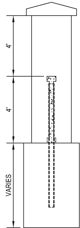
A-A 4' PANEL WITH 8' COLUMN SIDE ELEVATION
