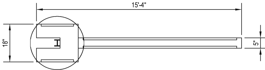
4' PANEL WITH 8' COLUMN TOP ELEVATION
