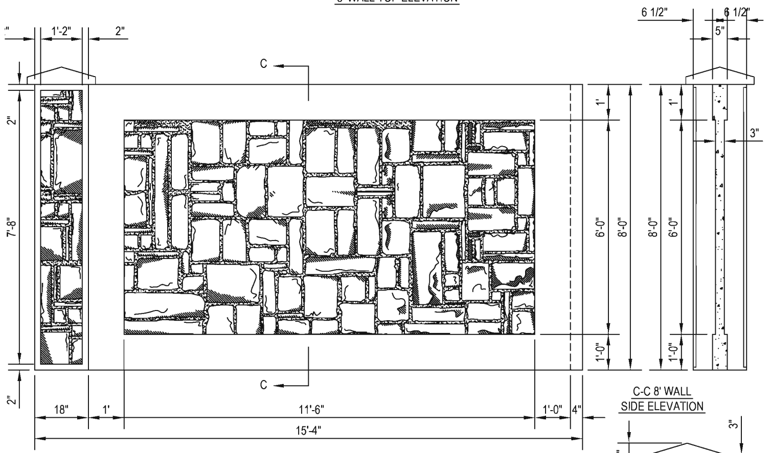
8' WALL ELEVATION
