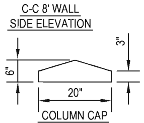
C-C 8' WALL SIDE ELEVATION
